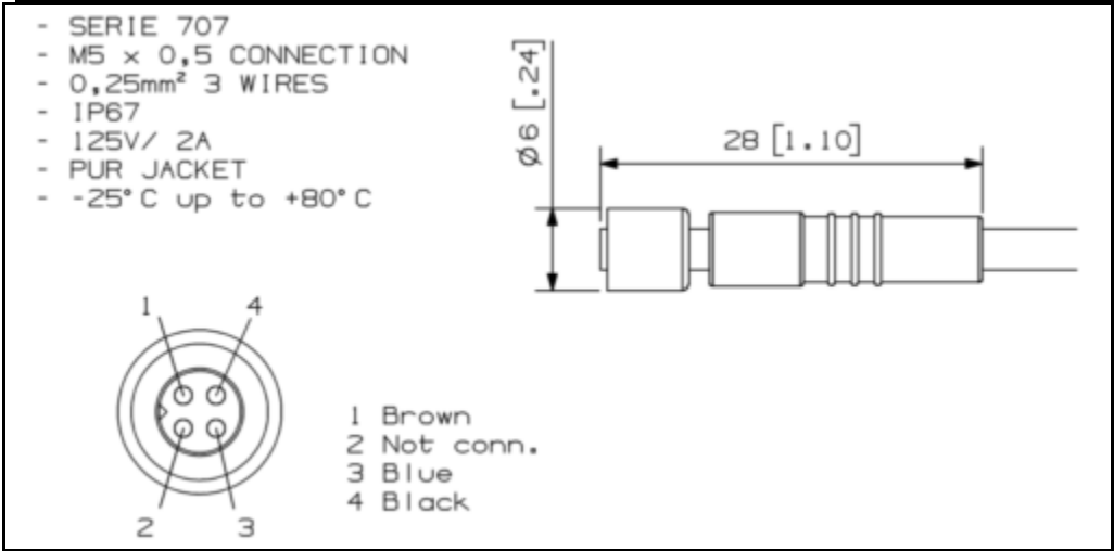
Figure 4-3 M5 Mating Connector and Cable Specifications
