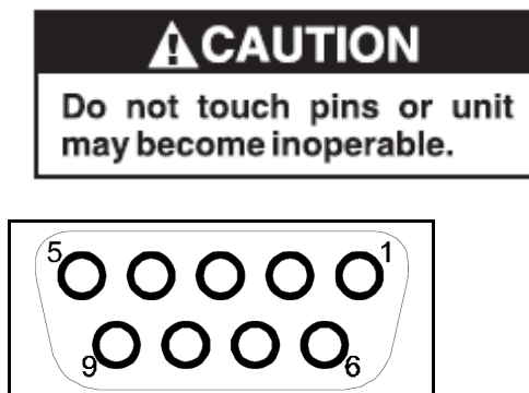
Figure 4-2 Profibus 9 pin D-sub connector
