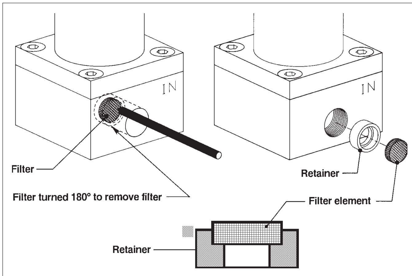
Figure 4-1 Filter Replacement
