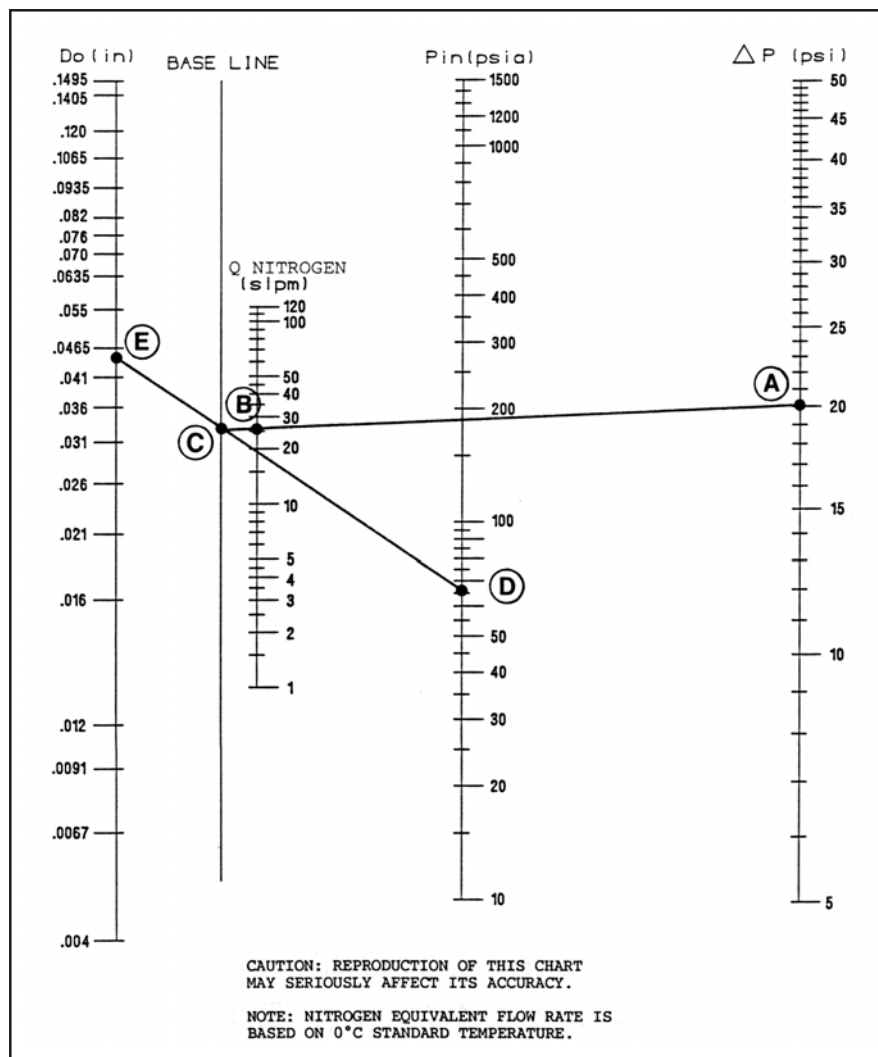
Figure 4-2 Example Nomograph
