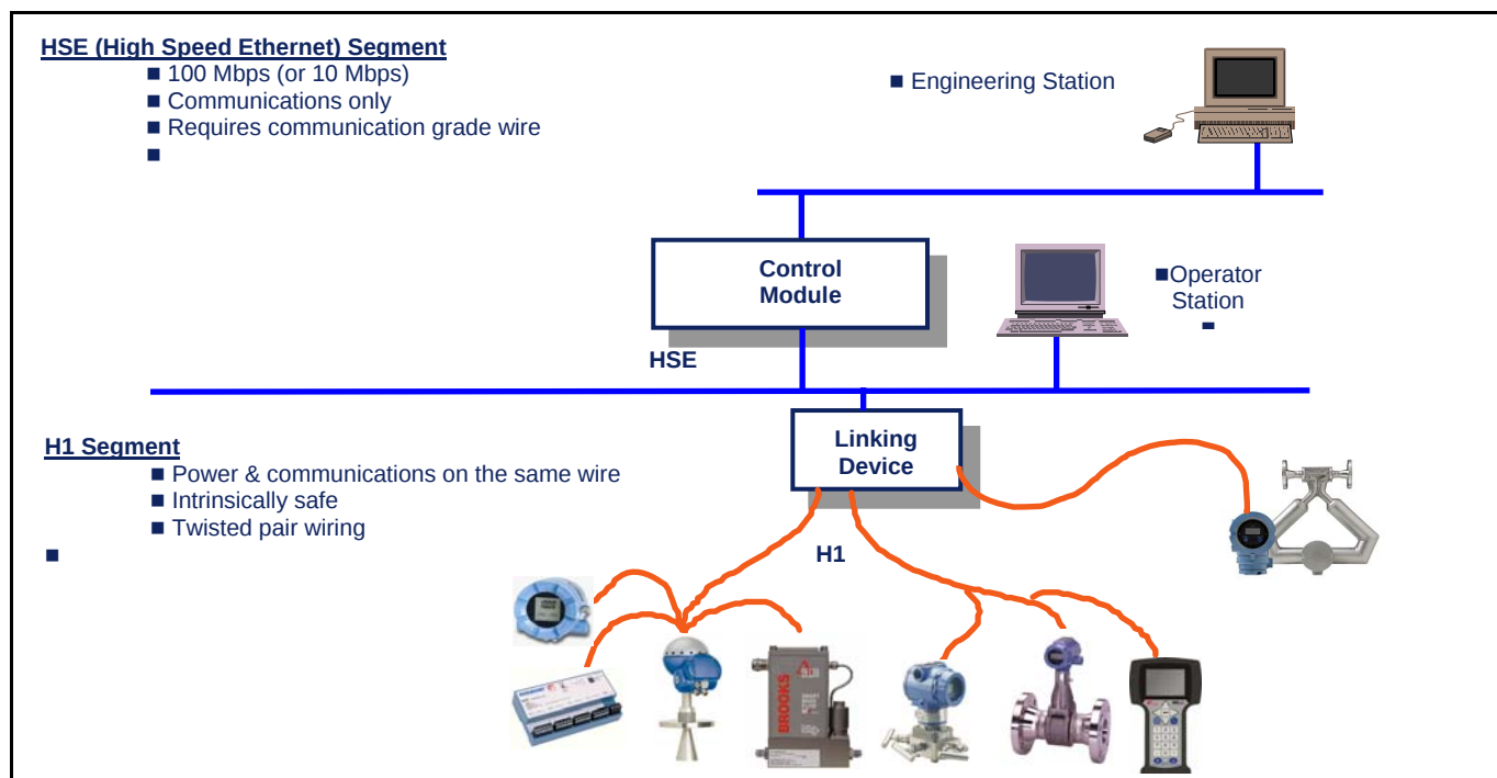
Figure 2-1 Typical FOUNDATION Fieldbus Installation
