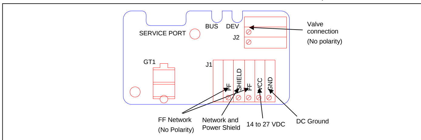
Figure 2-6 Terminals Board Connection
