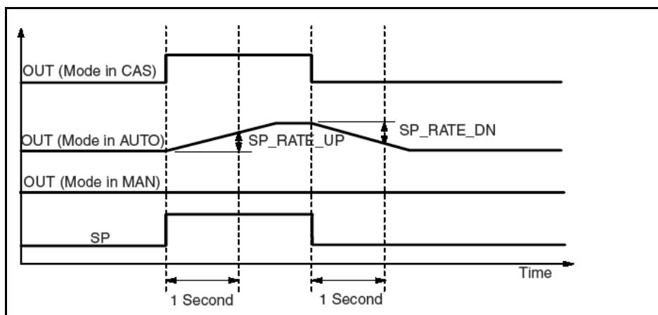
Figure 5-4 Analog Output Function Block Timing
