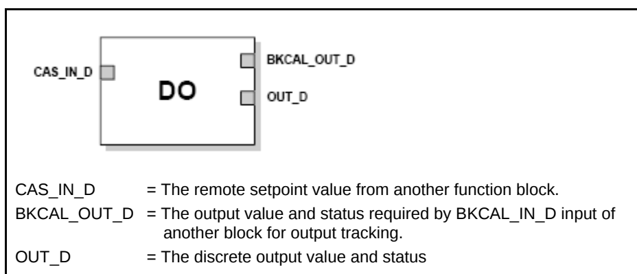
Figure 5-5 Digital Output Function Block
