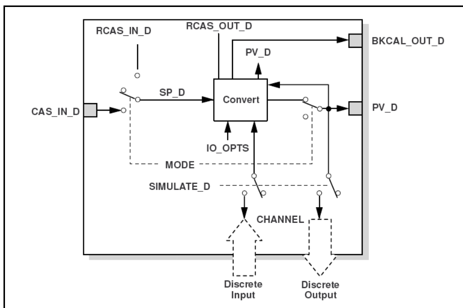
Figure 5-6 Discrete Input Function Block Schematic
