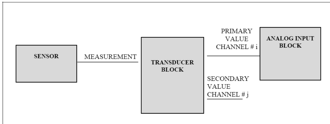
Figure 7-3 Temperature Transducer Block Schematic
