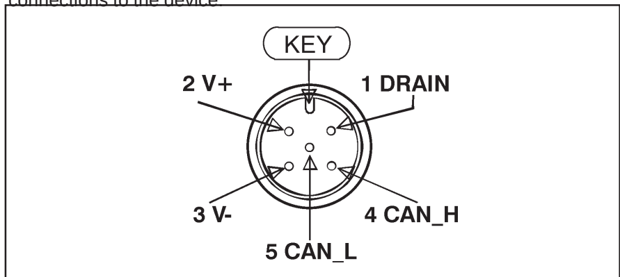
Figure 3-3 Interface Connector
